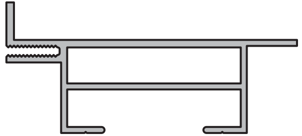
PREMARCO UNIVERSAL
