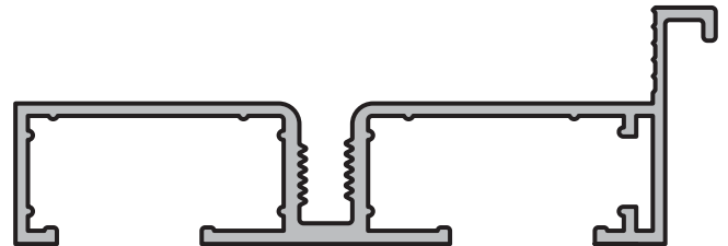
PREMARCO STANDARD
